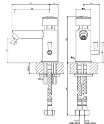
ACT210200 Self-closing basin mixer
