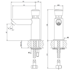
ACT220200 Self closing basin tap
