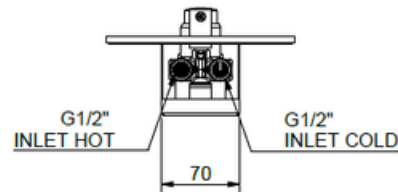
ACT060200MIX Self-closing built-in Shower Mixer with plastic box
