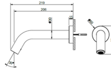
ACT901700 Wall mounted sensor spout
