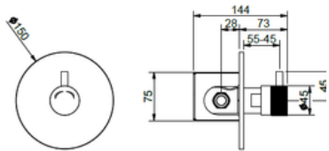
ACT060300MIX Self-closing built-in Shower Mixer with plastic box
